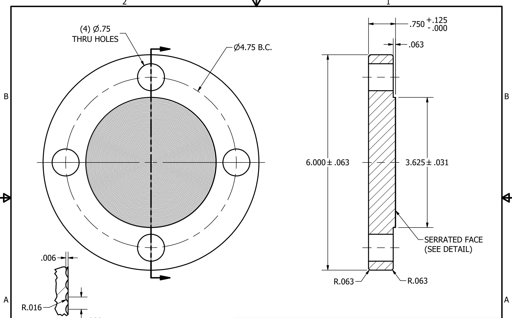
SERRATION DETAIL
